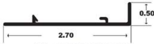
364 - DIRECT MOUNT 1"
