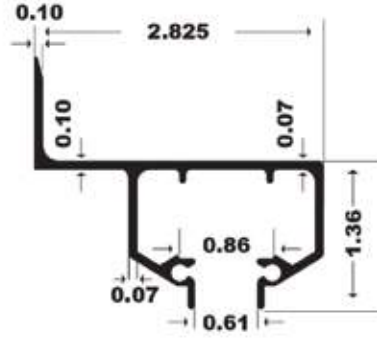
367 - 1" WALL HEADER
