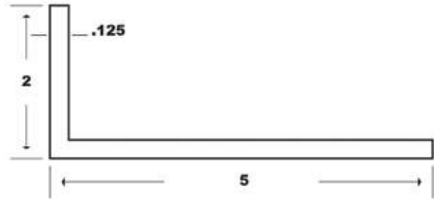
107 - 2" x 5" x .125 ANGLE
