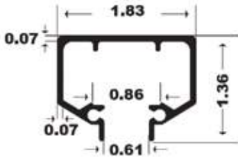
368 - CEILING HEADER
