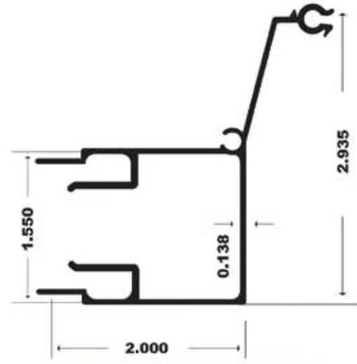
336 - HI TECH FEMALE CM
