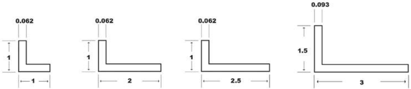
101 - 1" x 1" x .062 ANGLE
