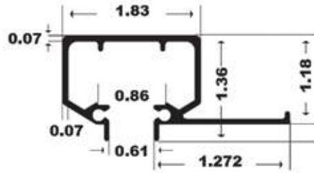
354 - CEILING HEADER RAINGUARD
