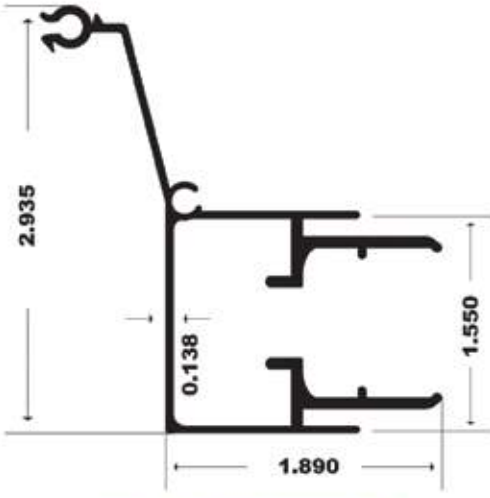
335 - HI TECH MALE CM
