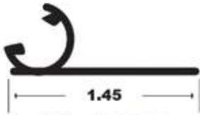
363 - STARTER
