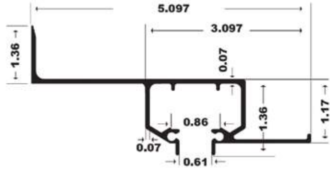
355 - 2" B/O WALL HEADER RAINGUARD
