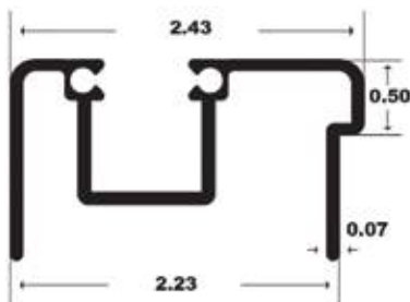
356 - ADJUSTABLE TOP
