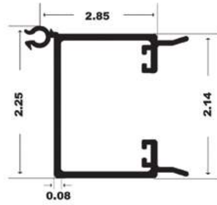
361 - COMMERCIAL C/M FEMALE
