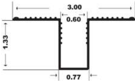
358 - RECESSED TRACK
