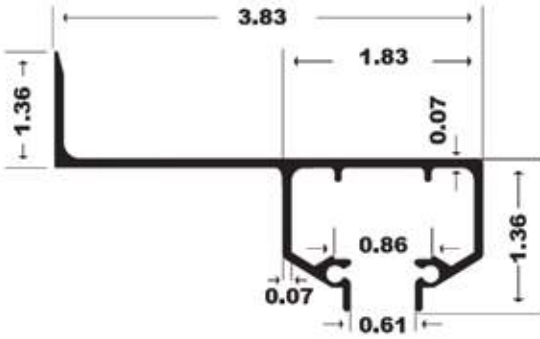
369 - 2" B/O WALL HEADER
