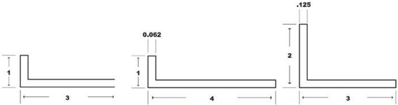
108 - 1" x 4" x .062 ANGLE
