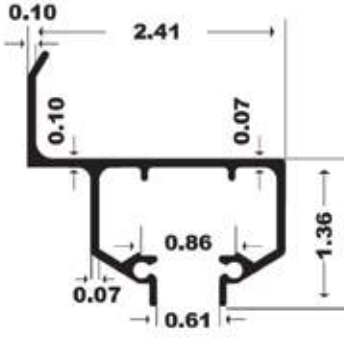
366 - 5/8" WALL HEADER
