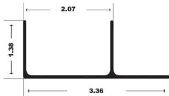
357 - ADJUSTABLE BOTTOM
