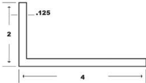
106 - 2" x 4" x .125 ANGLE
